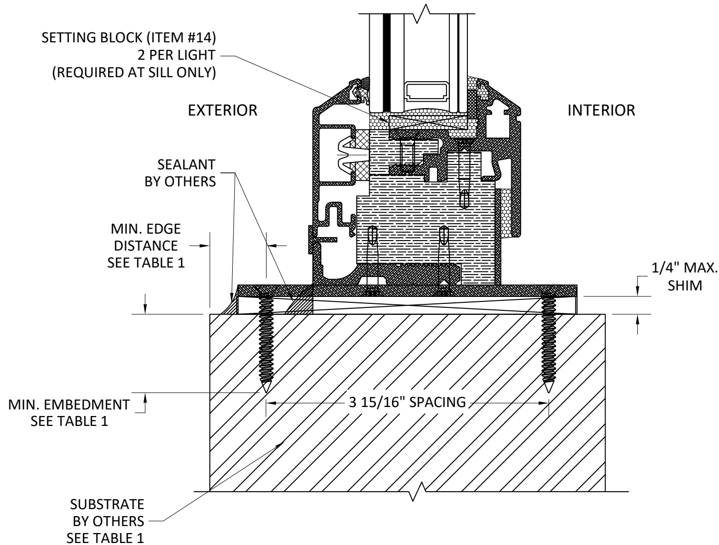
TYPICAL INSTALLATION (SILL/HEAD/JAMB)
